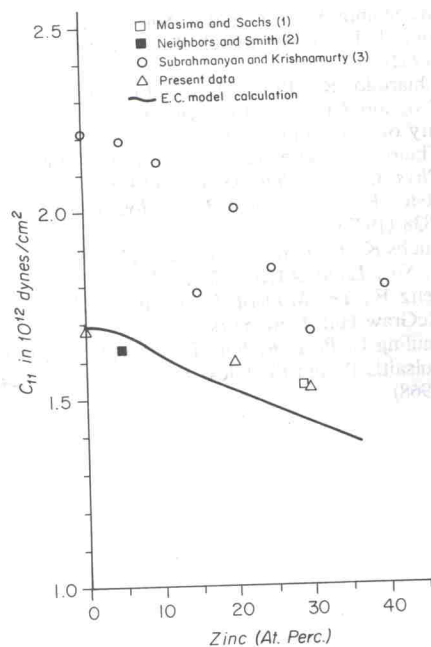
Fig. 3. Young's modulus as function of composition.
